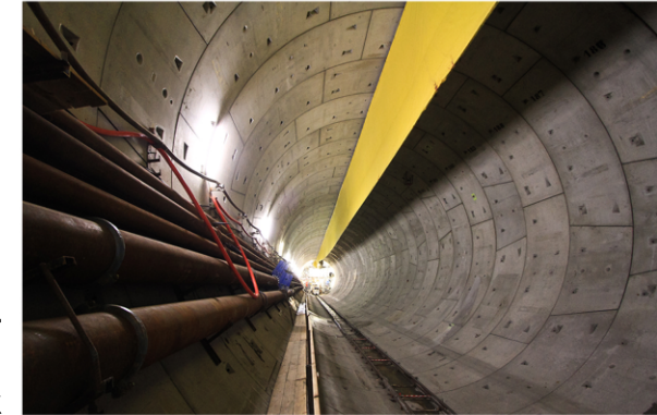
Tunnel under Martwa Wisła Gdańsk
